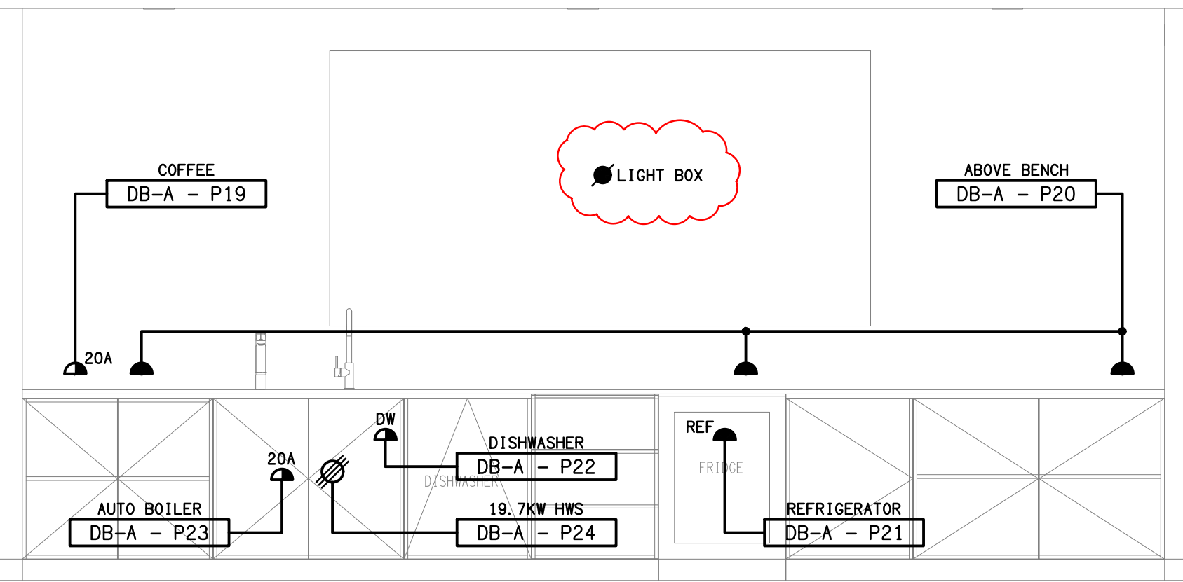
DETAIL A CUSTOMER LOUNGE KITCHENETTE ELEVATION SCALE 1:25
