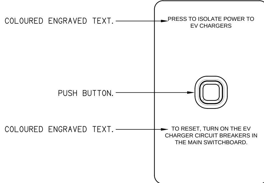
DETAIL B ELECTRIC VEHICLE CHARGING ISOLATION SWITCH (CIS) NOT TO SCALE
